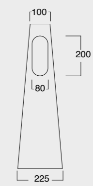
Cod. 35000101 Colonna Equilibrium scarico parete Column Equilibrium wall drain
